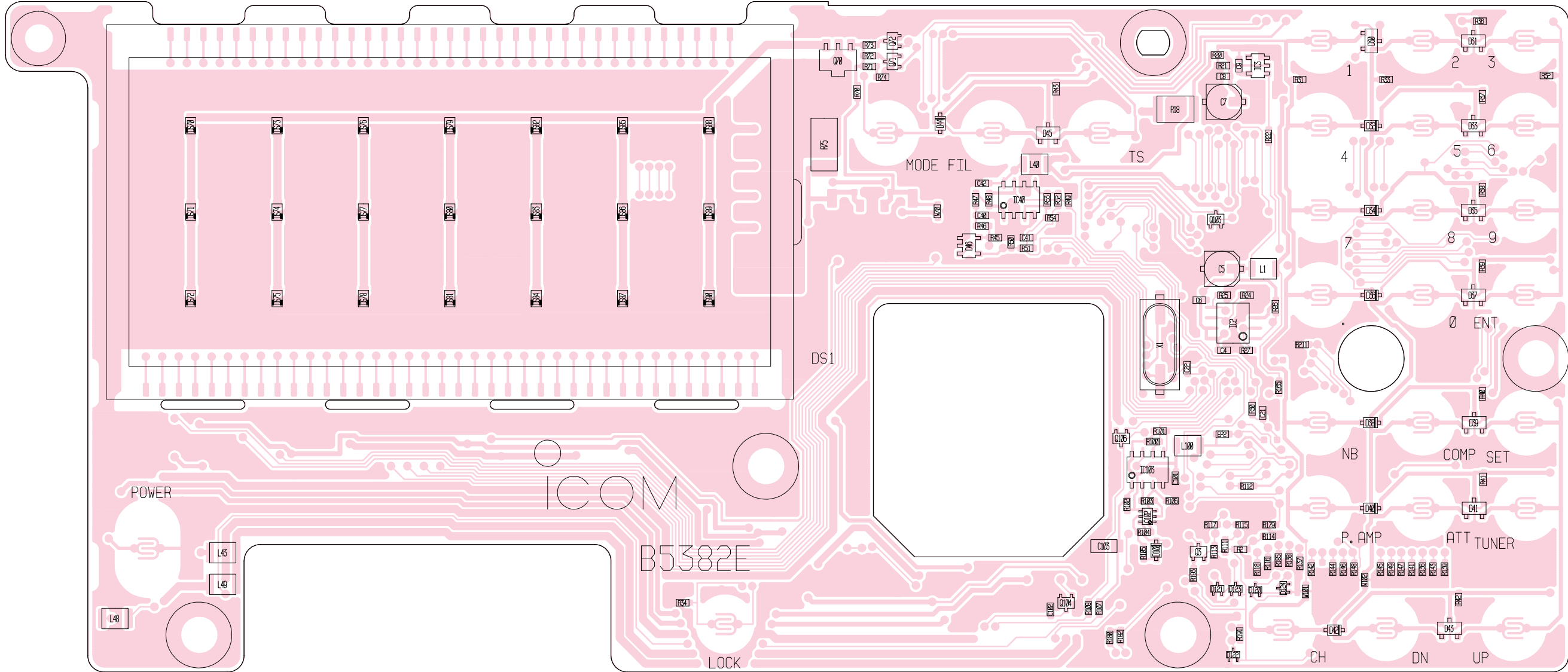
9-4 LOGIC UNIT • TOP VIEW
