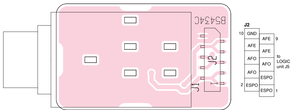
9-5 PHONE BOARD • TOP VIEW
