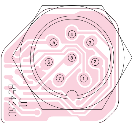
9-6 MIC BOARD • TOP VIEW
