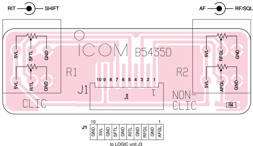
9-7 VR BOARD • TOP VIEW
