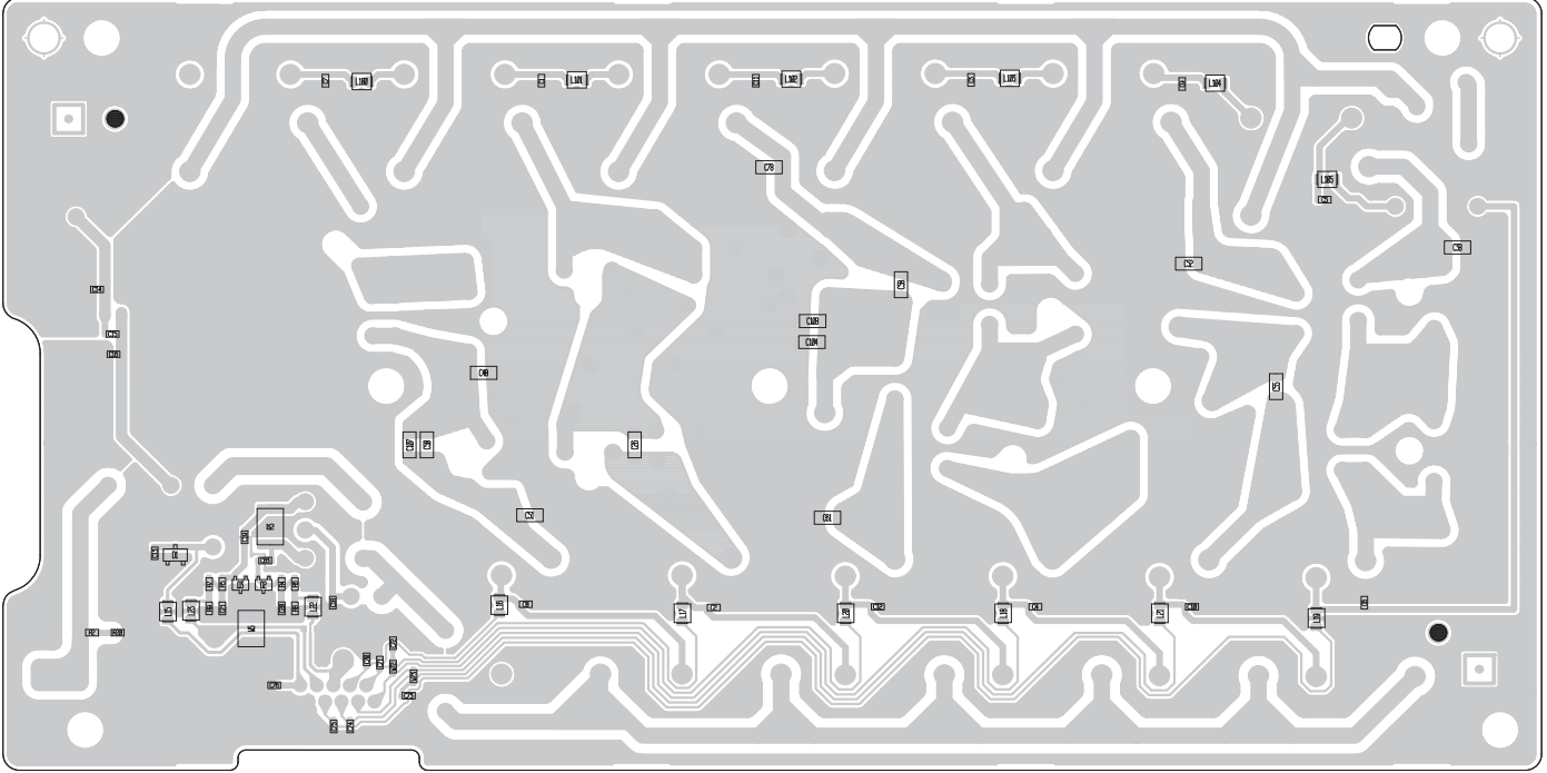
• FILTER UNIT (BOTTOM VIEW)
